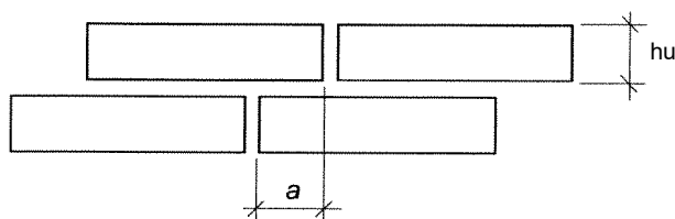
Figuur 1 – Overlappingslengte a
